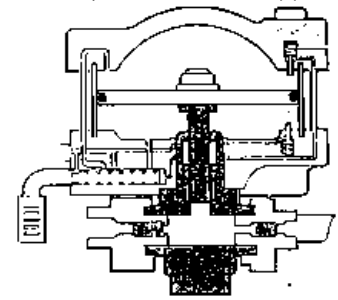
2. Hydraulic Section
