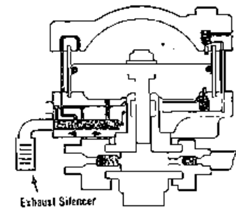
3. Air Cycling Valve Assembly
