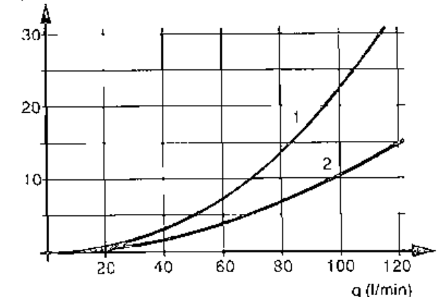
\Delta p (bar) Anti-cavitation characteristics
