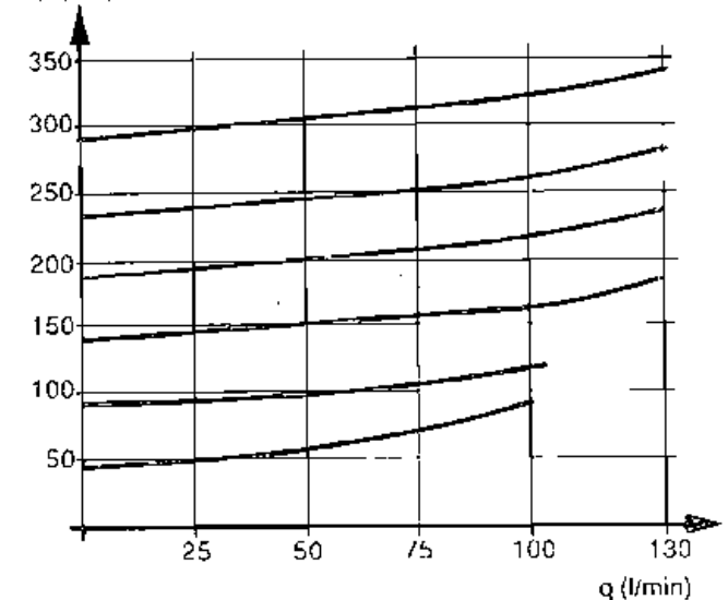
\Delta p (bar) Motor-port relief valve characteristics
