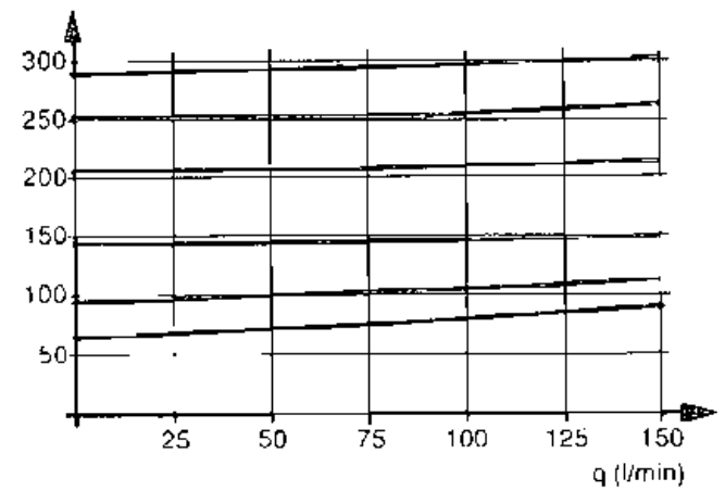
\Delta p (bar) Pressure relief characteristics
